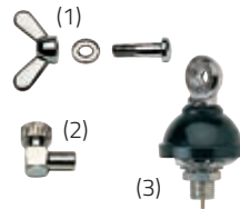
SC 27 T441 Specific screw (1) LC 27/10-N T370.01 Connector (2) FC 27 T478 Base for antennas (3)
