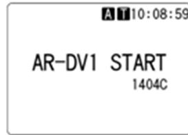
Opening screen
